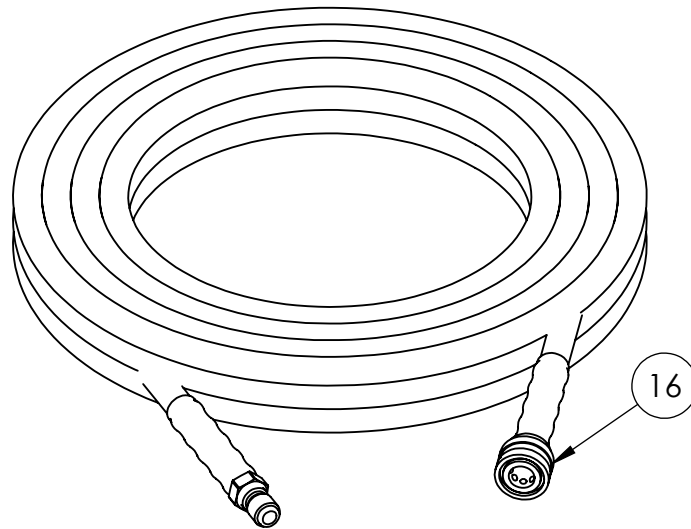
HOSE, 3/8" x 50' x 4500PSI 3/8" QC-M x 3/8" QC-F RUBBER PART NO. 7104844
