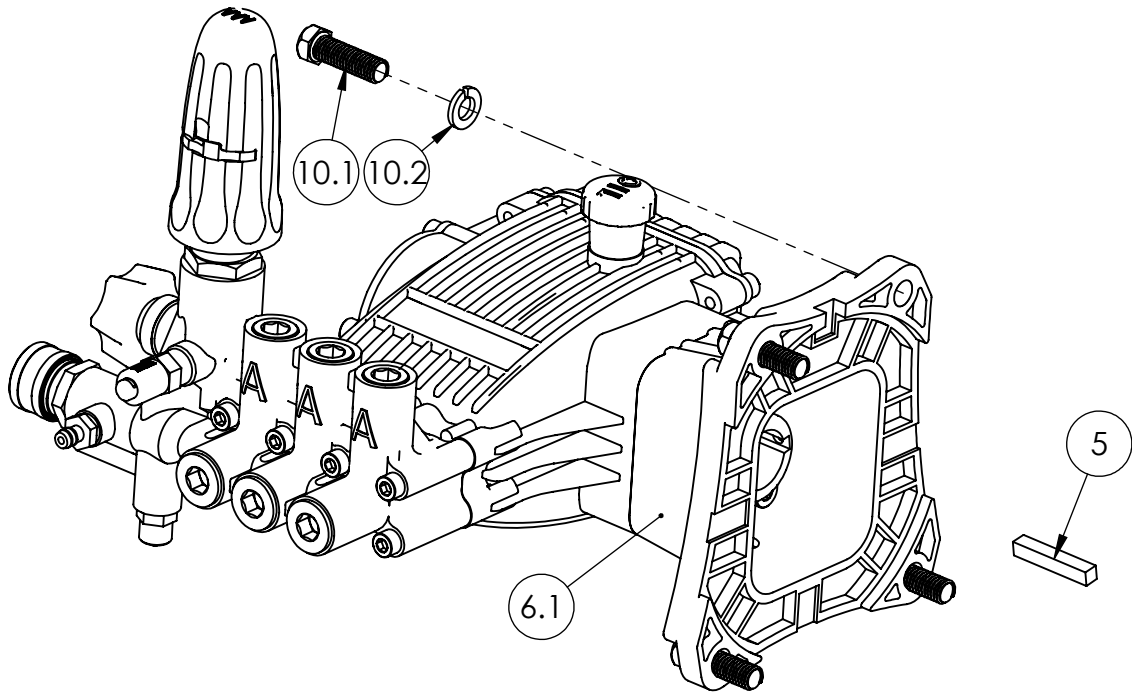
PUMP, ZWD-K4042 SERVICE KIT PART NO. 7105462
